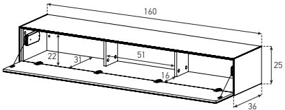
ED36F (WITH CABLE MANAGEMENT)
